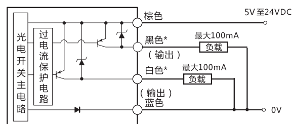
PNP
