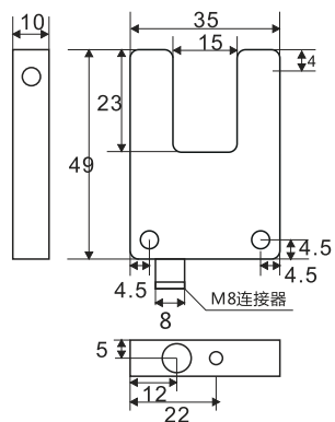
UC-SPM15N-M1
